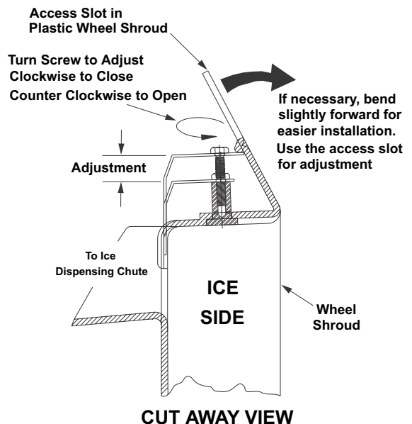
CUT AWAY VIEW
