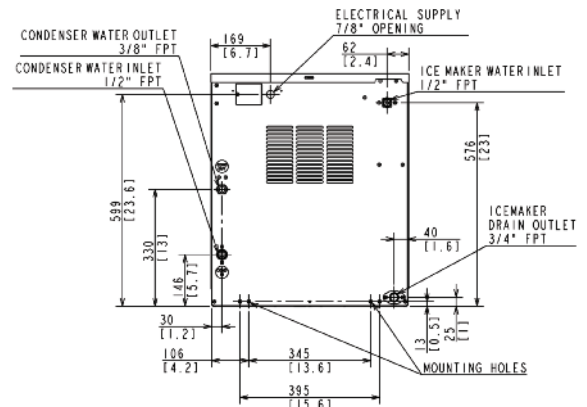
WATER-COOLED UNIT
